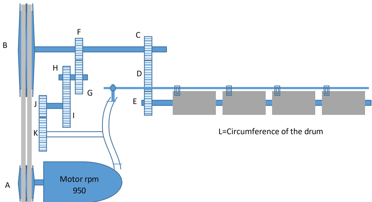
Typical Gearing Diagram of a Cheese winding machine
